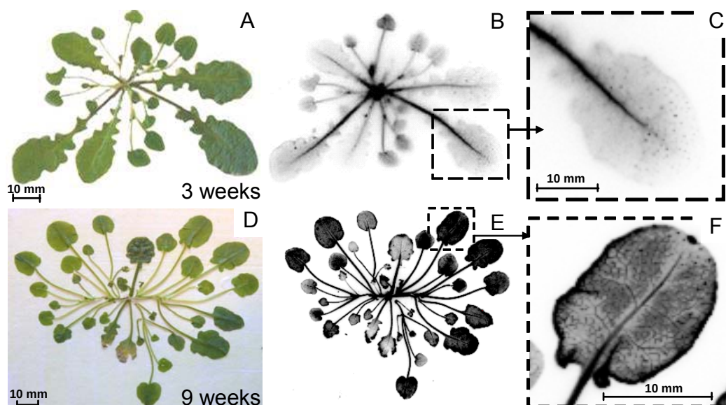
Figure 4: Photographs (A, D) and autoradiographs (B, E) of A. halleri MET exposed for 3 and 9 weeks to the ^{109}\text{Cd}_{20/30} treatment. On autoradiographs dark regions correspond to ^{109}\text{Cd} -enriched zones. Zooms on a mature leaf representative in terms of radioactive intensity are shown in (C, F). These zoomed images presented a treatment; indeed, the gray scale was adjusted in order to visualize the different compartments of the leaf.
