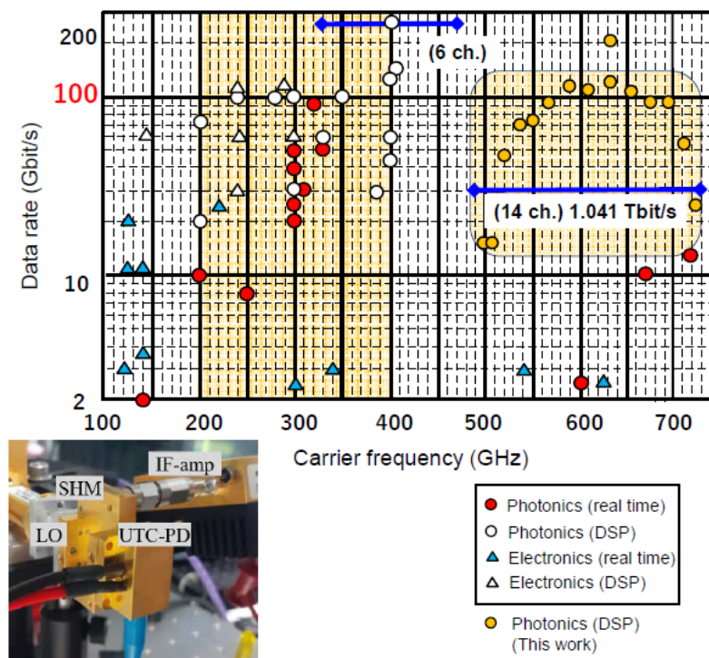
Figure.IV.17: Benchmark of the data-rate demonstrated using single carrier frequencies in the range 100-750 GHz. The photonics-electronics association in the WR1.5 shown here open new research routes for the use of the 600 GHz band. Inset: view of the UTC-PD module connected to the SHM.
