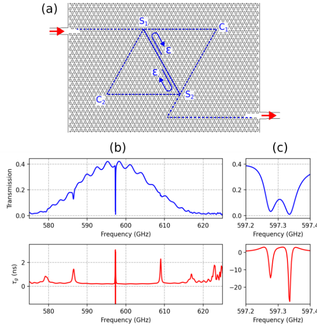
Figure. II.19: (a) Top view of the device with double-cavity resonator. Corners are labelled C1 and C2, splitters S1 and S2. The parameter \epsilon is the reflection coefficient on the splitter, for an edge mode propagating along the common edge S1S2 of the double cavity. (b) Transmission spectra (top) and group delay (bottom) as a function of the frequency; (c) same as (b) for a frequency range closer to the split resonance at 597 GHz.
