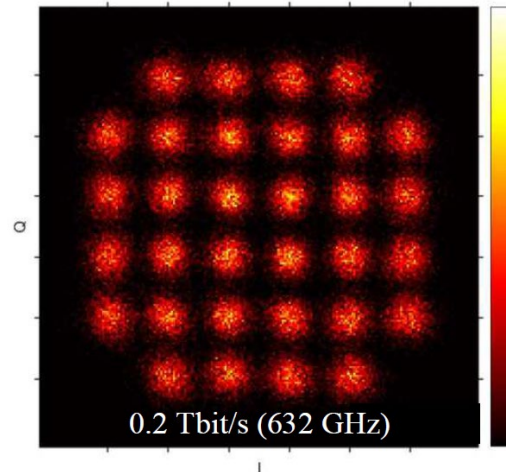
Figure IV.16: I/Q map of single channel 0.2 Tbit/s at 632 GHz. BER is 1\text{E-}2 , below SD-FEC limit.
