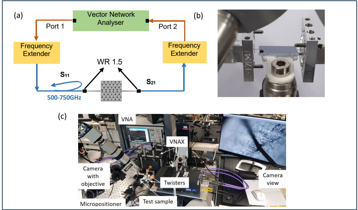
Figure IV.3 : Experimental Setup (a) S parameters measurements experimental setup schematic (b) View of the coupling of the topological devices to hollow-core waveguide measurement interfaces. (c) View of the total experimental setup in the laboratory
