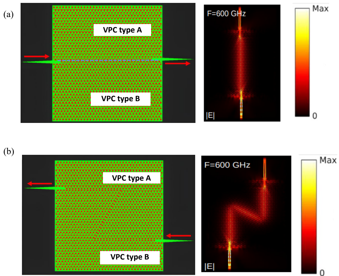
Figure II.12(a): Schematic of the bent waveguide designed using triangular holes and magnitude of the electric field confined at 600 GHz (b) Schematic of the bent waveguide designed using triangular holes and magnitude of the electric field confined at 600 GHz
