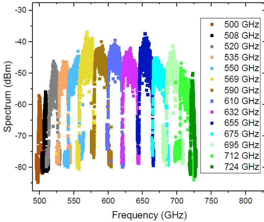
Figure. IV.12. Measured spectra, from IF analysis, at oscilloscope input.
