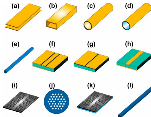
Figure I.8: Low-loss waveguides for the THz range, (a) parallel plates waveguide, (b) metallic rectangular waveguide, (c) metallic circular waveguide, (d) circular waveguide with dielectric coating, (e) polymer fiber, (f) coplanar showing substrate in aquamarine color, (g) slot line, (h) stripline, (i) photonic crystal waveguide, (j) photonic crystal fiber, (k) SIIG with dielectric substrate, (l) ribbon waveguide. The colors gray, yellow, and blue represent silicon metal, and low-index dielectric material, respectively. [69]
