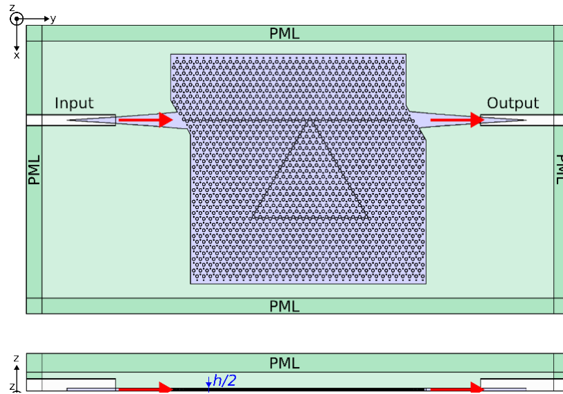
Figure. II.16: Numerical setup for finite elements simulations of the full membranal device. The thickness of the membrane is h=90\mu\text{m} , the dielectric constant of silicon is 11.7.
