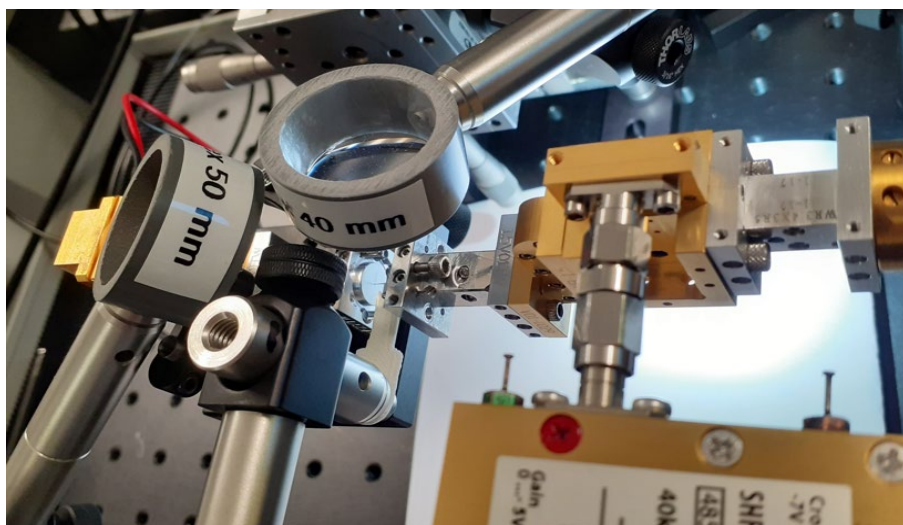
Figure. IV.19: Experimental View of the 600GHz datacom testbed
