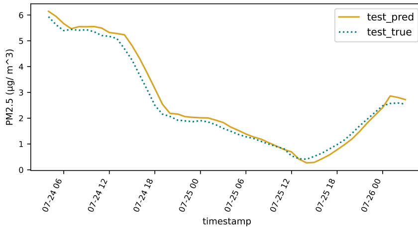
Figure 3.4: Hourly temporal prediction of PM_{2.5} levels over time over the Canal site, forecasting 2-day predictions for July 24th (Saturday) and July 25th (Sunday), 2021. The golden solid line represents the predicted values and the dotted green line represents the truth values for the test set.
