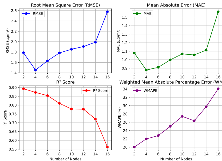
Figure 5.19: Evaluation of our model’s performance with four metrics: RMSE, MAE, R^2 , and WMAPE on an unseen dataset across different node configurations.
