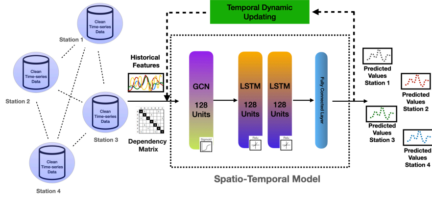
Figure 4.2: Proposed spatiotemporal model. The model incorporates GCN blocks for capturing spatial features, LSTM blocks for capturing temporal features, temporal dynamic updating blocks, input data, a dependency matrix representing spatial relationships, and the predicted outputs.
