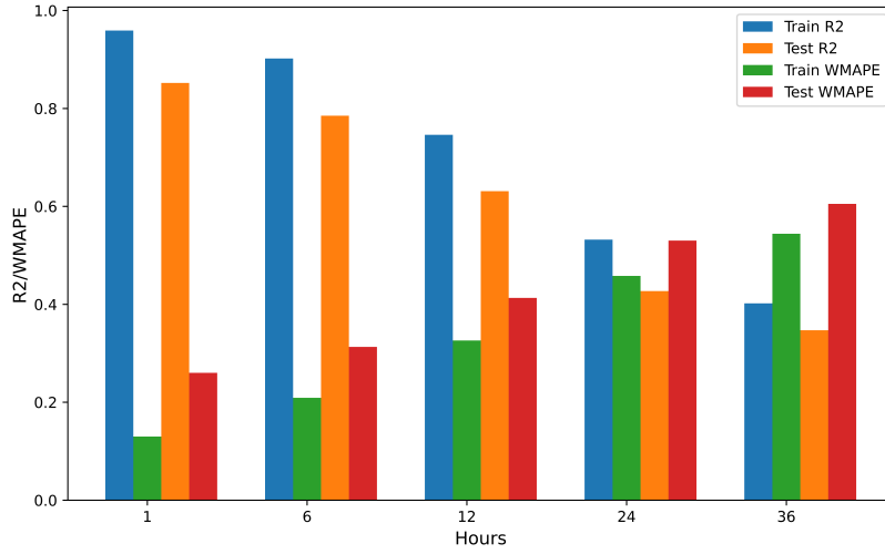
Figure 4.9: Performance Evaluation of Long-Term \text{PM}_{2.5} Forecasting with GT-LSTM presents the R^2 and WMAPE metrics, showing a decrease in accuracy over time. Blue and green bars represent the training set metrics, while orange and red bars correspond to the test set metrics. Accuracy is assessed using both R^2 and WMAPE.
