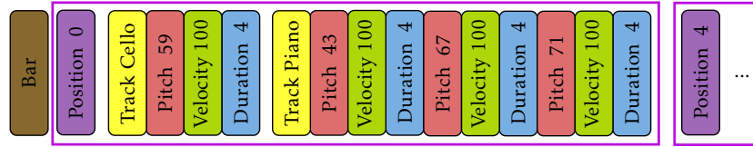
(c) REMI+ with vertical parsing (beat-first).
