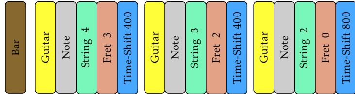
Figure 4.4: Elementary tokens examples. (a) Time can be encoded following a performance-based paradigm, where music is represented as successive performance events (<note-on>, <note-off>). (b) Instead, time can be encoded following a score-based paradigm, with music is organized along a metrical time grid structured by bars and beats. (c) Event-based tokenization can also be specific to particular instrumental notations, such as guitar tablatures.
