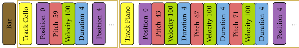
(b) REMI+ with horizontal parsing (track-first).
