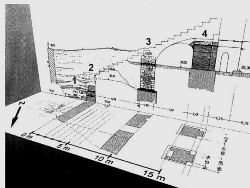
Fig. 8.24 Byzantine remains at the northwest corner of the Hippodrome.
