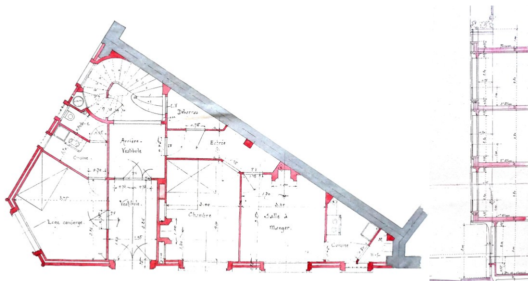
Figure 3.7: Original architectural designs for the immeuble at 185 rue Belliard, Paris (Deneux, 1913) with floor plan and section showing the use of the adapted Cottancin system and hollow exterior walls, 1910. (Archives de Paris, as adapted by Gillet 2020, p.220)
