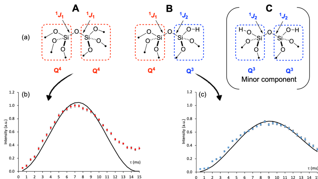
Figure 5 (a) Structure of local siloxane environments. (b,c) Build-up curves of ^{17}\text{O}\{^{29}\text{Si}\} DFS- J -HMQC-QCPMG signals at (b) 34 and (c) 22 ppm assigned to siloxane sites. The red points and the blue squares correspond to the experimental data, whereas the black lines are the simulated curves. The build-up curves were obtained by averaging 10624 transients for each of 30 t_1 increments with a recycle delay \tau_{\text{RD}} = 0.5 s, leading to an experimental time of 45 h. The red and the blue points correspond to the experimental data, whereas the black lines are the simulated curves. The errors bars in the experimental curves subsume the contributions of the noise standard deviation and the error due to the nonlinear fit with DMFIT 46 .
