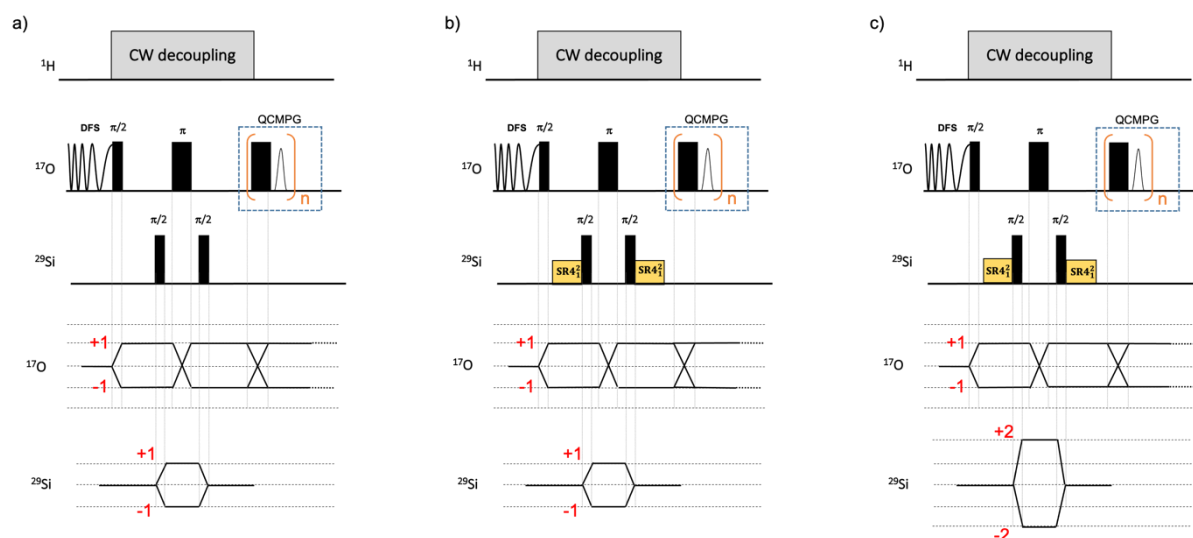
Figure 2. ^{17}\text{O} - \{^{29}\text{Si}\} DFS-HMQC-QCPMG pulse sequences using coherence transfers via ^{17}\text{O} - ^{29}\text{Si} (a) J - or (b,c) dipolar coupling. The coherence transfer pathways for ^{17}\text{O} and ^{29}\text{Si} channels are shown at the bottom of the figure. For the D -HMQC sequences, we selected via phase cycling either (b) single-quantum (SQ) and (c) 2Q ^{29}\text{Si} coherences during the indirect evolution period, t_1 . The pulse programs of pulse sequences (b) and (c) are given in the Appendix 2 of the Supporting Information.
