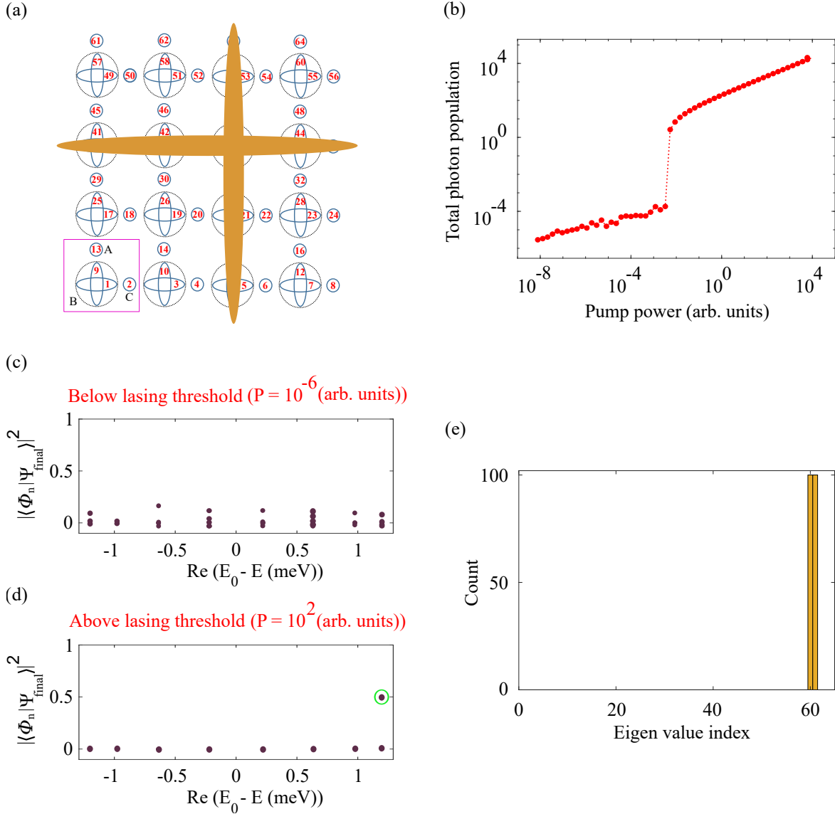
Figure 5.5: (a) Sketch of the configuration for the excitation of crosspump of the lattice. (b) Total photon population as a function of pump power, showing the onset of lasing. The final steady-state photon wavefunction projected onto the eigenmodes ( |\langle \Phi_n | \Psi_{\text{final}} \rangle|^2 ) at two pump strengths, one below (c) and one above the lasing threshold (d). (e) Histogram of the lasing eigenmodes across 100 different realizations showing two eigenvalue index lasing simultaneously.
