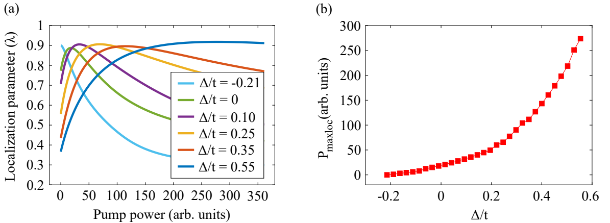
Figure 3.5: (a) Numerical results for the \lambda dependence on pump power for the same detuning settings as in the experiments in Fig. 3.4, with g_x \neq 0 . (b) Maximum localization power ( P_{\text{maxloc}} ), as a function of detuning \Delta/t .
