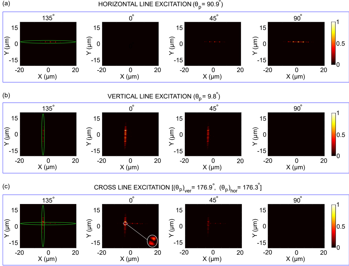
Figure 4.10: Real space photoluminescence (PL) images analyzed at four output polarization angles: 135^\circ , 0^\circ , 45^\circ , and 90^\circ , using a polarization analyzer consisting of a half-wave plate and linear polarizer. (a) PL from the horizontal line with horizontal spot excitation at P = 35\text{mW} . (b) PL from the vertical line with vertical spot excitation at P = 35\text{mW} . (c) PL under cross pumping excitation with a total power of 71\text{mW} . All images are extracted at a fixed energy slice (top sp band).
