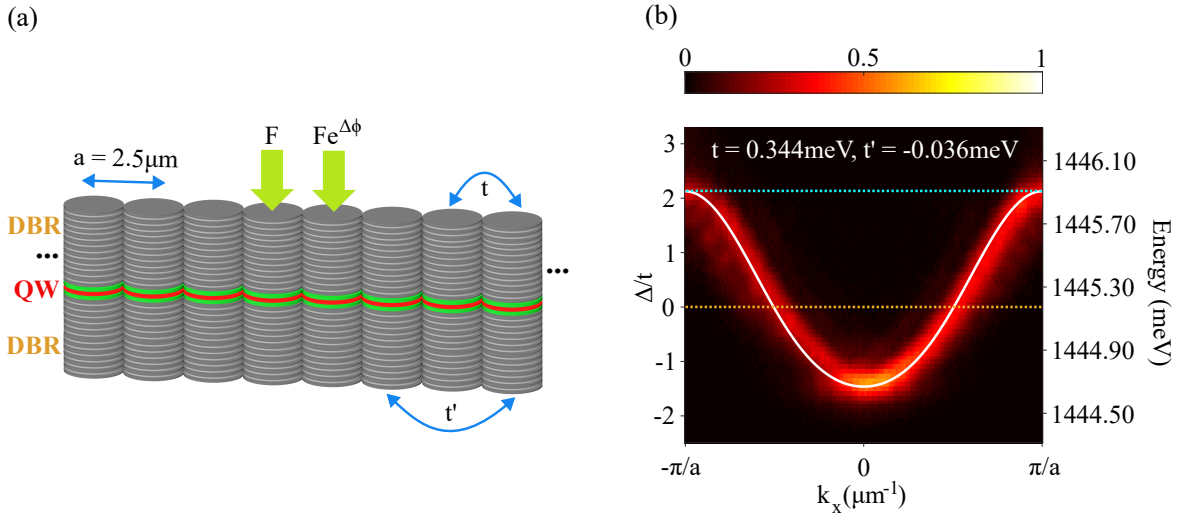
Figure 2.1: a) Schematic representation of the one-dimensional lattice consisting of 31 micropillars with a center-to-center separation of a = 2.5\mu\text{m} . The excitation spots are placed on adjacent pillars, with equal amplitudes F and a phase difference \Delta\phi . (b) Angle-resolved photoluminescence measurement of the 1D lattice with one pump spot, showing the energy bands as a function of the in-plane momentum k_x , with \Delta = E_p - E_0 , where E_0 = 1445.13\text{meV} . The white line represents the fitted two coupled exciton-photon model. The blue and orange dashed lines indicate the laser energy pumped at the top of the band ( \Delta/t = 1.87 ) and at zero energy ( \Delta/t = 0 ), respectively.
