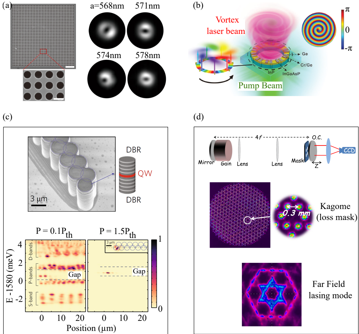
Figure 0.4: (a) SEM images of the BIC laser array ( a = 563 \text{ nm} , 40 \times 40 unit cells; scale bars 3 \mu\text{m} and 500 \text{ nm} ) and measured far-field patterns of symmetry-protected BIC modes for different a . Taken from [53] (b) Schematic of the OAM microlaser on an \text{InP} substrate with simulated spiral phase of the emitted light (OAM charge l = 1 ). Taken from [54] (c) Topological micropillar laser based on a zigzag chain of coupled micropillars embedding QWs between DBRs, showing lasing from a topological edge mode in the bandgap. Taken from [55] (d) Degenerate cavity with a masked gain medium imaged onto a back mirror in a 4f telescope. A kagome-shaped loss mask selects \sim 1500 coupled Gaussian beams forming a 2D kagome laser lattice. The far-field interference recorded on a CCD shows broad bow-tie features instead of sharp peaks, revealing frustrated phase locking and the absence of long-range phase order. Taken from [56].
