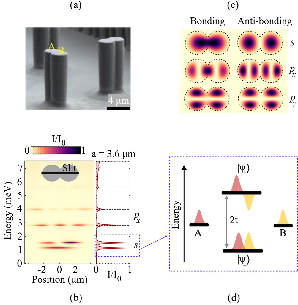
Figure 1.7: (a) SEM image showing two etched micropillars brought close together to form a dimer. (b) Spatially resolved photoluminescence spectrum measured from a dimer with radius R = 2\ \mu\text{m} and separation a = 3.6\ \mu\text{m} . The inset indicates the position of the spectrometer slit, and the dashed line corresponds to finite-element calculations for the same geometry. (c) Intensity patterns of the six lowest eigenmodes for a = 3.6\ \mu\text{m} , arranged according to their single-pillar orbital type and their bonding or antibonding character. (d) Sketch illustrating how the two lowest s -modes hybridize into bonding ( |\psi_+\rangle ) and antibonding ( |\psi_-\rangle ) states. All the images in this figure was taken from [125].
