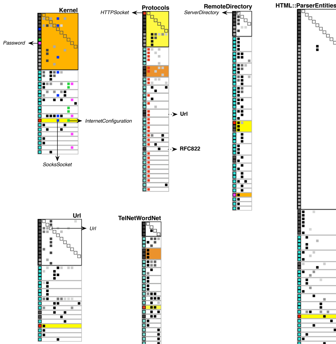
Figure 3.8: Outgoing reference blueprints of some packages of the Network system. In this view, the Kernel package was selected in orange, surfaces with Protocols package are highlighted in yellow, class HTTPSocket in red, class SocksSocket in blue, class InternetConfiguration in green, and class Password in fuchsia.
