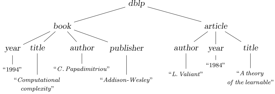
Figure 1.1: A trivialized DBLP repository.
