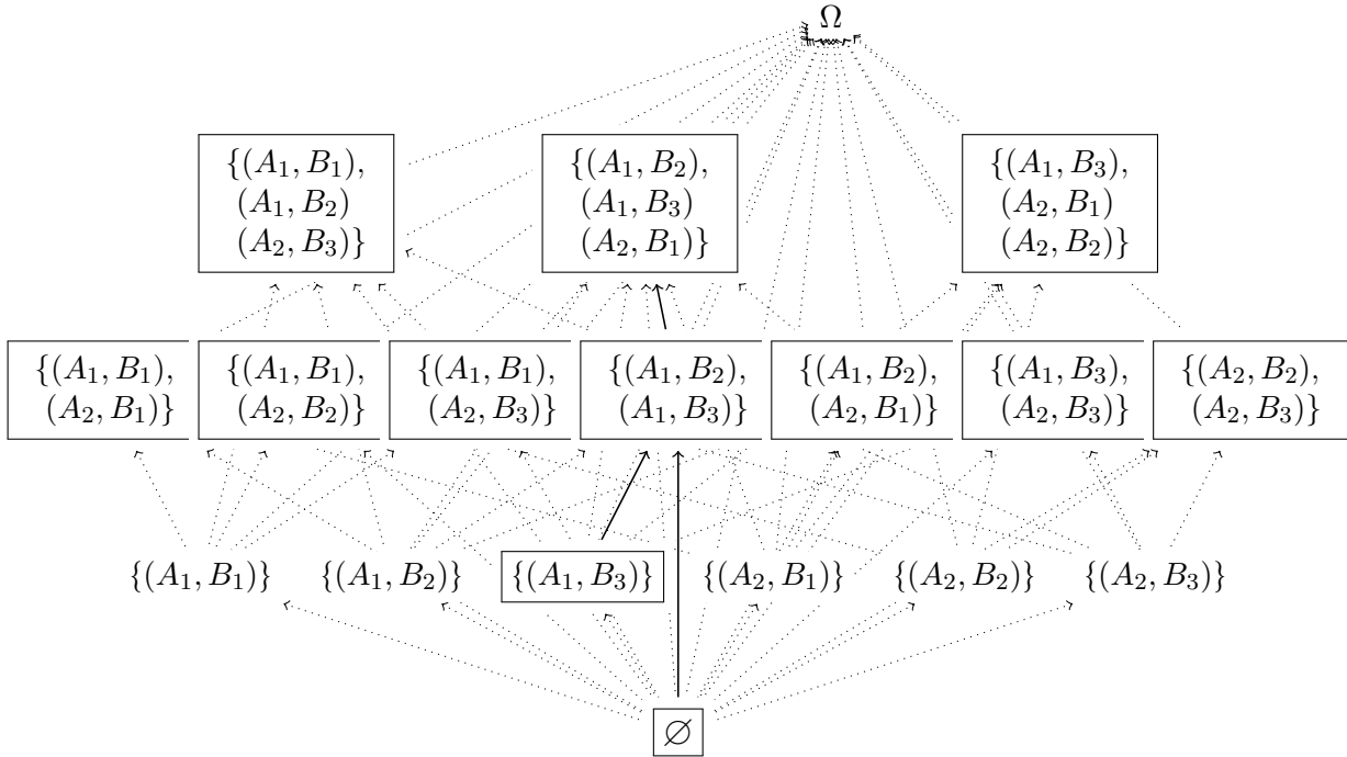
Figure 4.5: Lattice of join predicates for the instance from Example 4.2.1.
