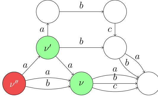
Figure 5.9: Graph from the proof of Theorem 5.3.5.
