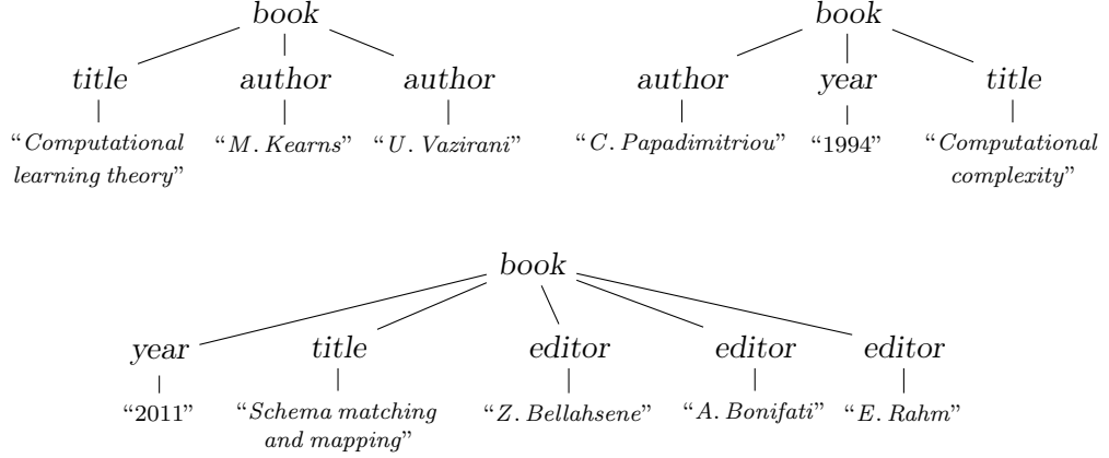
Figure 3.1: Three XML documents storing information about books.
