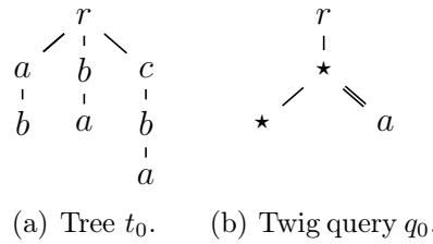
Figure 1.2: A tree and a twig query.
