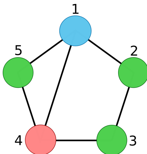
Figure 5: Exemple de graphe non orienté contenant 5 noeuds.
