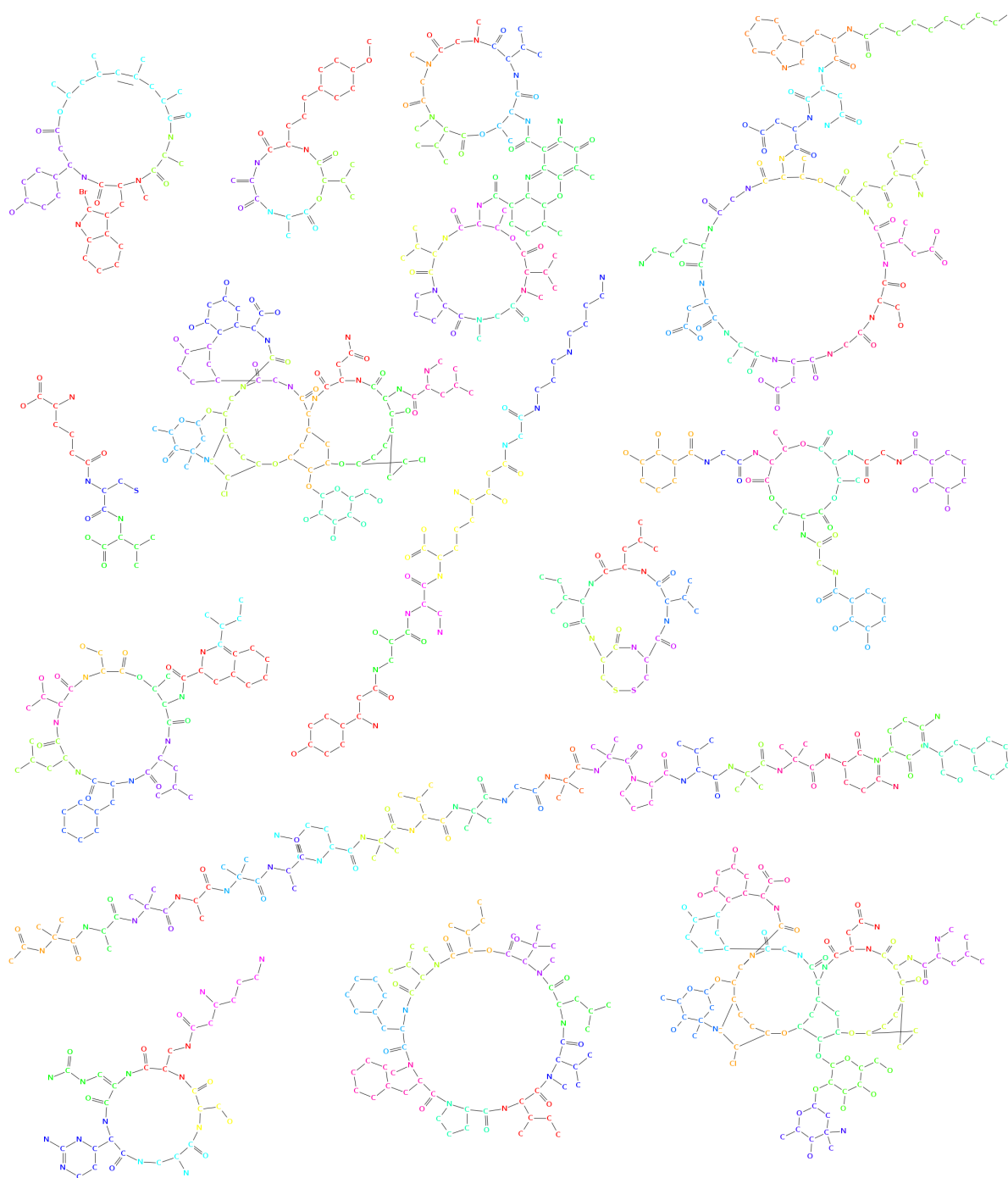
Figure 1.8: Patchwork de NRP
