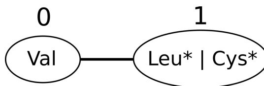
Figure 3.3: Requête Val,[Cys*|Leu*]@1@0.
