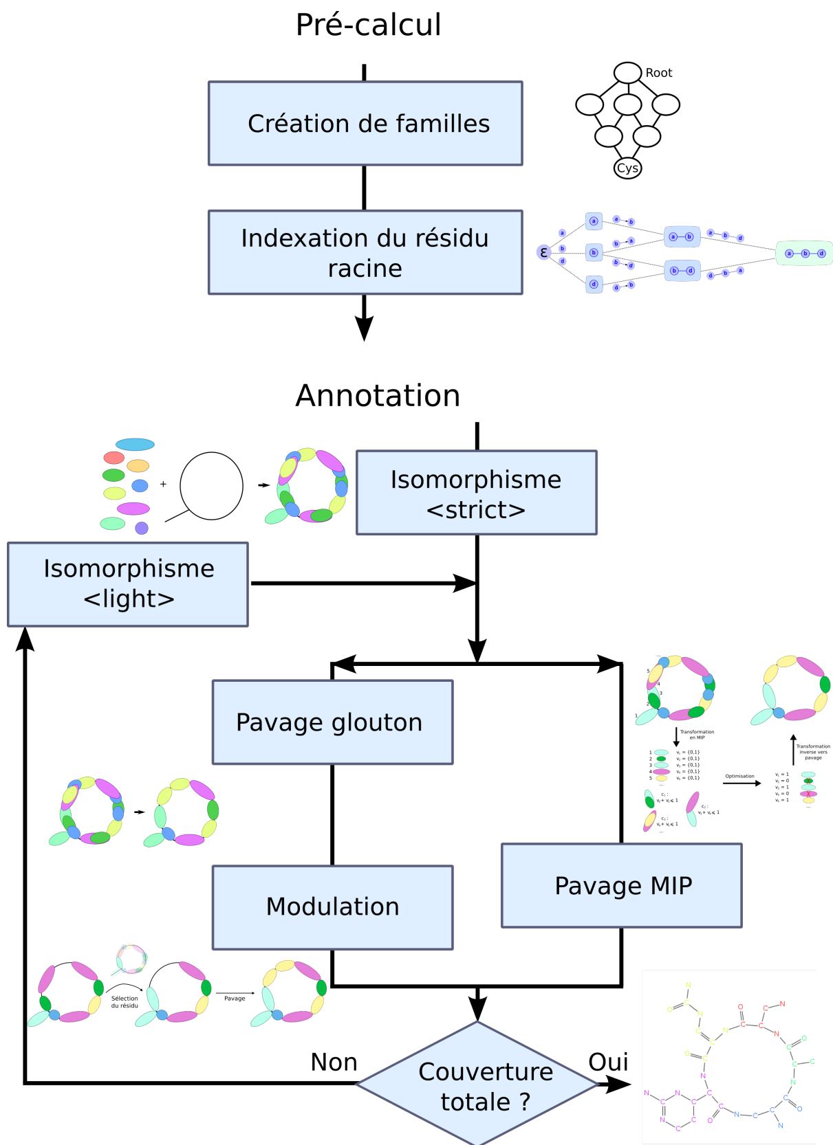
Figure 2.33: Schéma global de Smiles2Monomers
