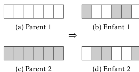
FIGURE 5.6 – Croisement uniforme.
