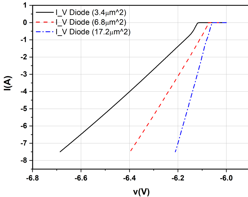
FIG. 2.26: I-V characteristics of 3 diode structures.
