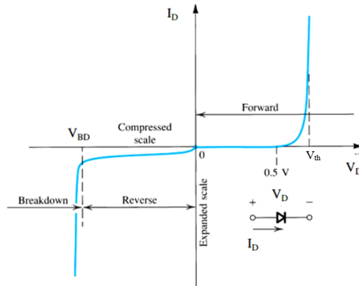
FIG. 1.13: I-V curve of a diode showing the avalanche break down.
