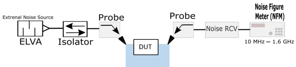
FIG. 2.1: Bench setup dedicated for noise measurements on D-band.
