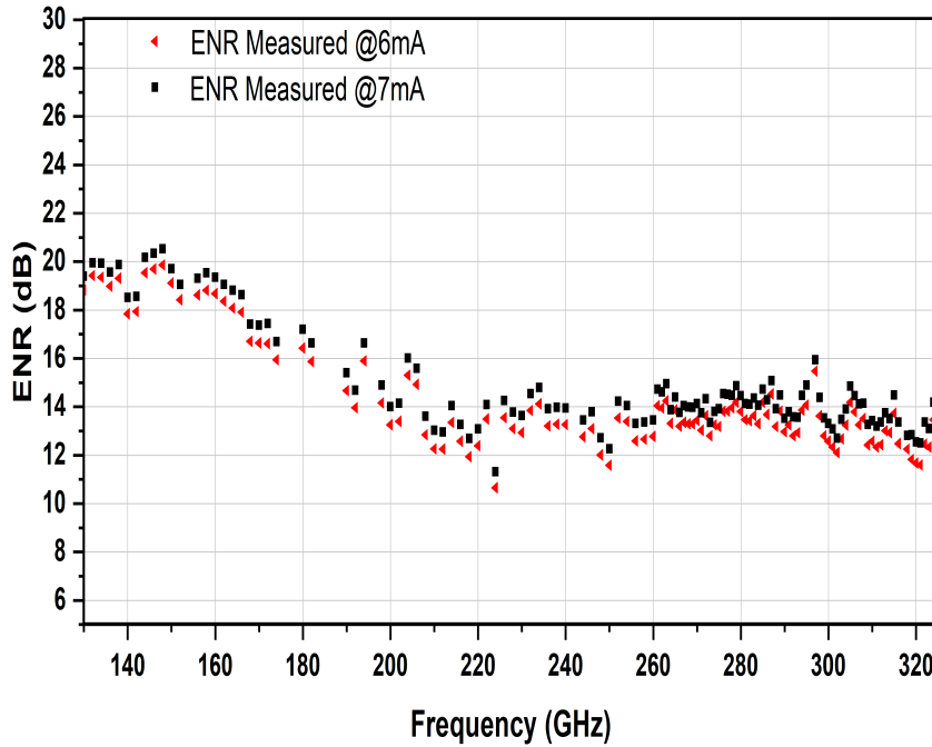
FIG. 2.22: Extracted ENR of the integrated noise source up to 325 GHz.
