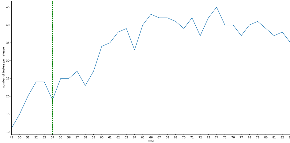
FIGURE 5.16: Number of testers per release.
