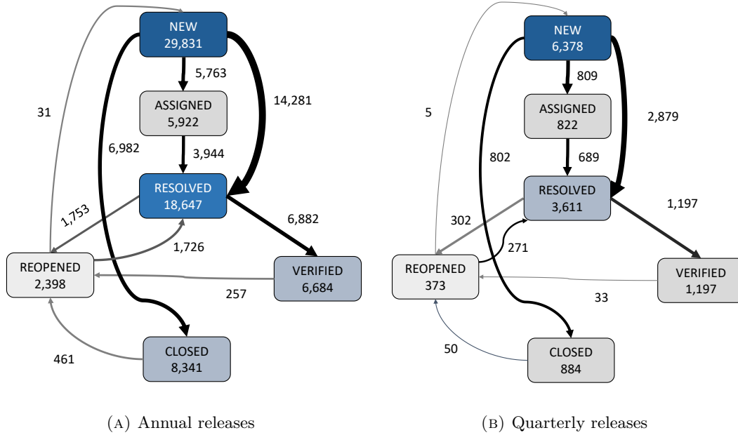
FIGURE 4.4: Process maps computed based on the event logs of the extracted Bugzilla bug reports for the Eclipse annual and quarterly releases.
