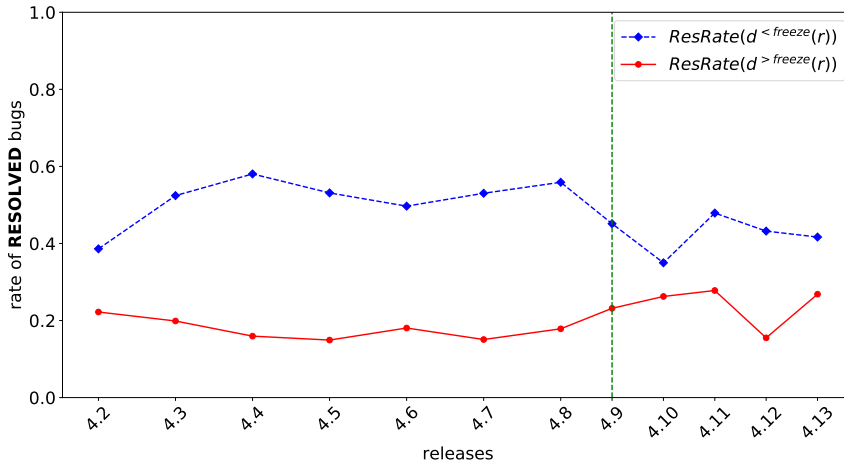
FIGURE 4.16: Evolution of \text{ResRate} during the development and feature freeze period for each 4.x release.
