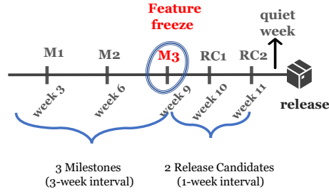
FIGURE 4.2: Quarterly release schedule for releases of Eclipse Core projects since 4.9.
