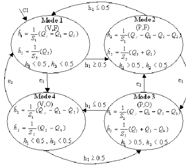
FIG. 6.2: Automate hybride
