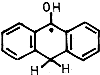
RADICAL HYDROXY-9-DIHYDRO- 10 ANTHRYLE-9
