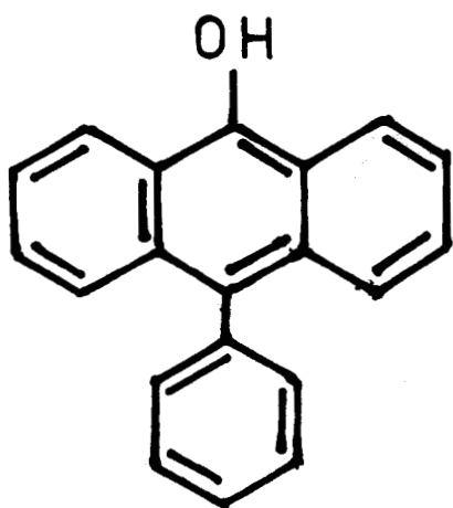
PHENYL ANTHRANOL
