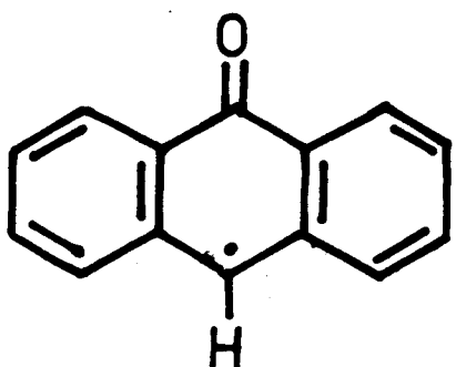
RADICAL ANTHONYLE III
