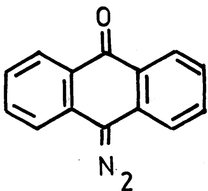
DIAZOANTHRONE I
