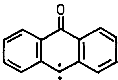
CARBENE ANTHONYLIDENE II
