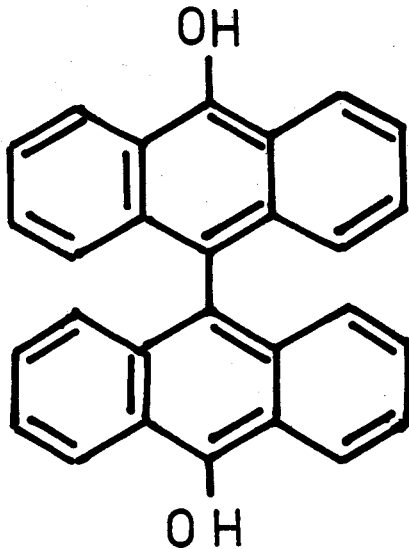
BIANTHRANOL
