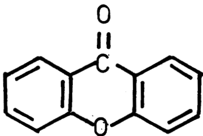
XANTHONE
