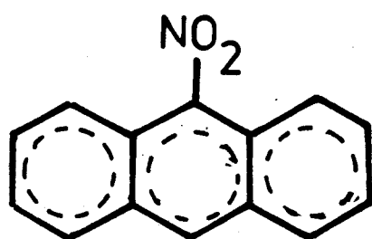
NITROANTHRACENE XVI
