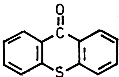
THIOXANTHONE XIII
