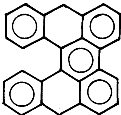
9,16 DIHYDRO DIBENZO [a,d] PERYLENE
