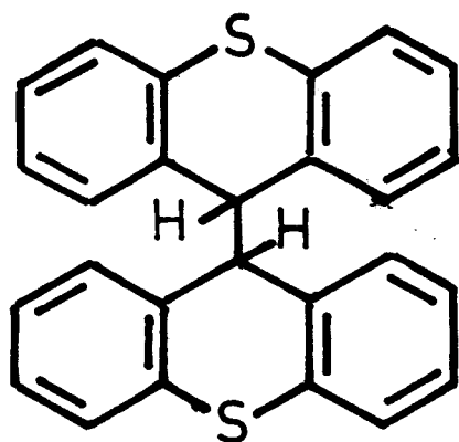
BITHIOXANTHYLE XV
