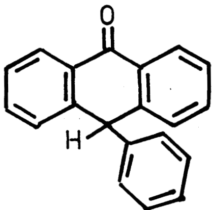
PHENYLANTHRONE
