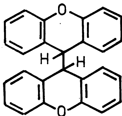
BIXANTHYLE XIV
