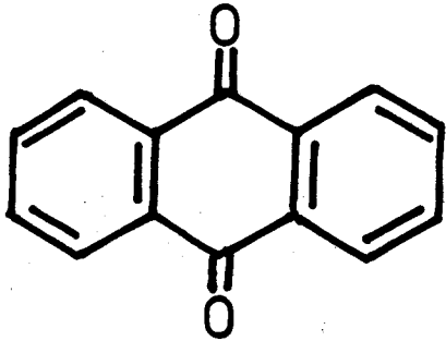
ANTHRAQUINONE
