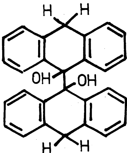
ANTHRAPINACOL
