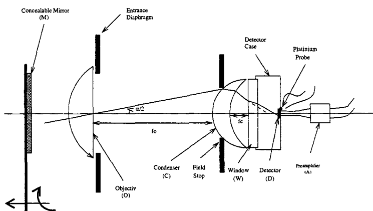
Figure 1: Optical front end of the instrument
