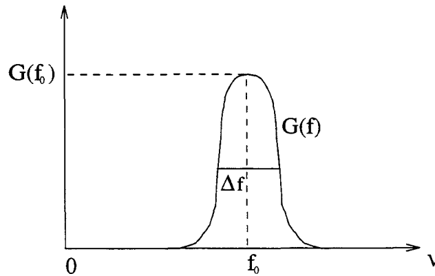
Figure II.4: Filtrage
