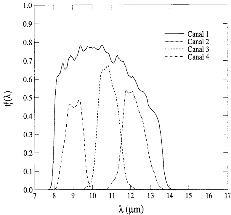
Figure III.6: Fonctions de transmission spectrales du prototype CLIMAT: Canal 1: [8,14 \mu\text{m} ], Canal 2: [11.5,12.5 \mu\text{m} ], Canal 3 [10.5,11.5 \mu\text{m} ], Canal 4: [8.2,9.2 \mu\text{m} ].
